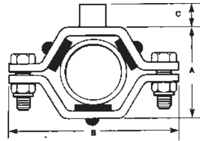
C24T Tubing Hanger (w/ 3/8" - 18NPT thread)
