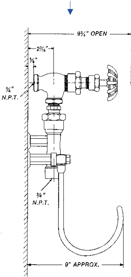
ANGLE VALVE - BACK ENTRY
